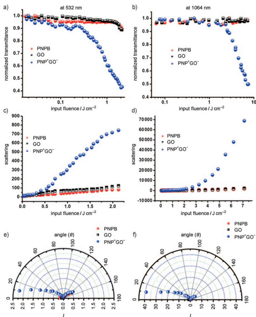
Figure 4. Optical limiting response of aqueous solutions of \text{PNP}^+\text{GO}^- ( 20 \text{ mg L}^{-1} ), GO ( 34 \text{ mg L}^{-1} ), and PNPB ( 2 \times 10^{-6} \text{ M} ), measured with 7 ns laser pulses at a) 532 and b) 1064 nm. Nonlinear scattering response of \text{PNP}^+\text{GO}^- , GO and PNPB solutions at laser pulses of 532 (c and e) and 1064 nm (d and f), where c) and d) show intensity-dependent scattering signals at 532 and 1064 nm, respectively, and e) and f) angle-dependent scattering signals at 532 and 1064 nm respectively.
